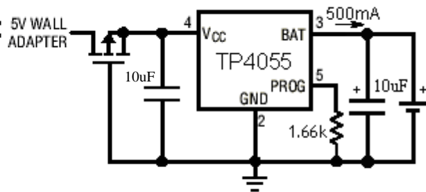
Charger with input reverse polarity protection
